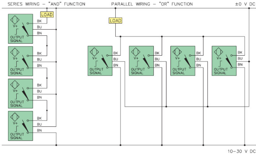
Figure 22 PNP Connection
