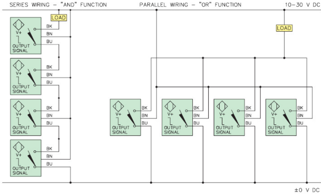
Figure 21 NPN Connection
